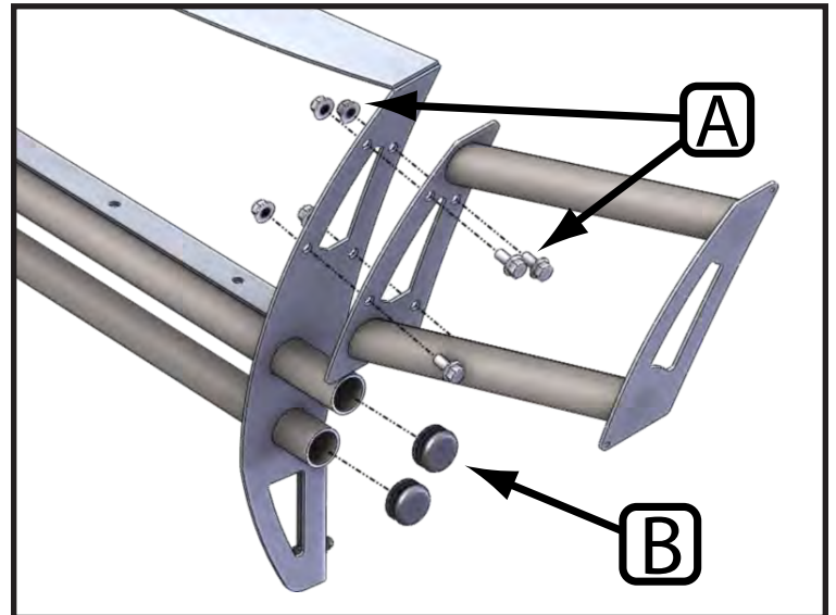
"Figure 2" Light Guard & Tube Cap Install
