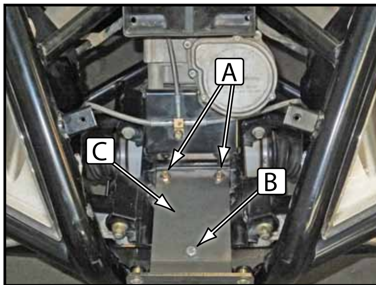
"Figure 3" Grill Bracket Install
