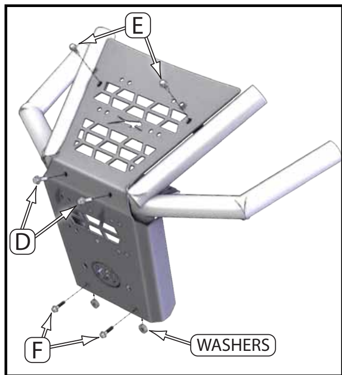
"Figure 4" Grill Plate Install
