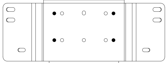
Wide 4 Hole Winch Pattern (6.6" x 3")
