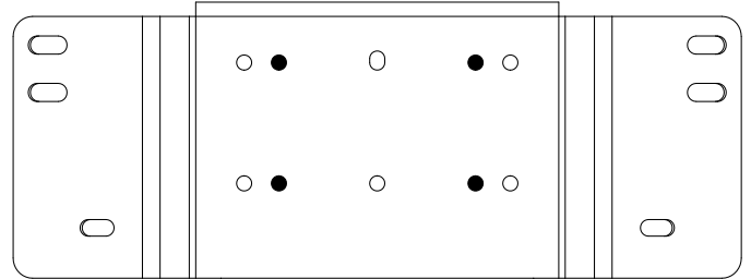
Standard 4 Hole Winch Pattern (4.875" x 3")
