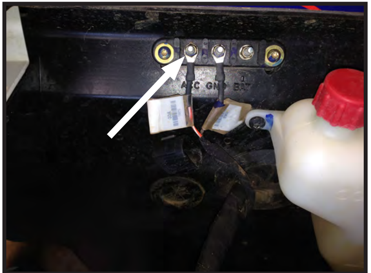
“Figure 15” Wire Location (Located under the hood.)
