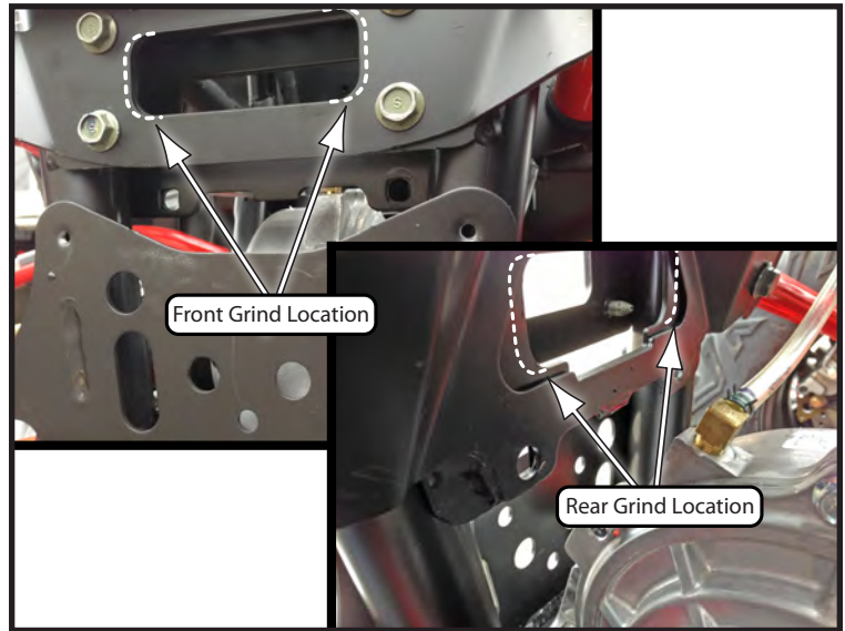
"Figure 5" Wide Winch Frame Modification
