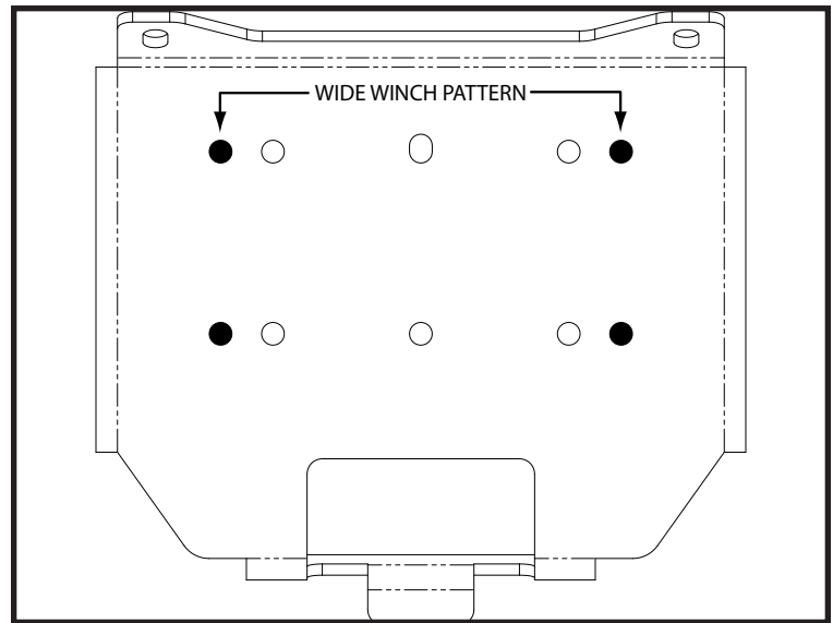
“Figure 9” Mount Hole Pattern
