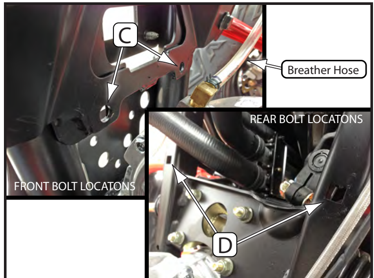
"Figure 6" Winch Mount Bolt Locations
