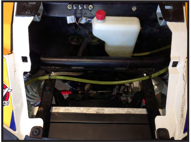
“Figure 13” Contactor Location (Located under the hood.)
