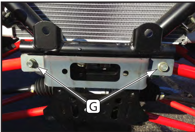
“Figure 12” Fairlead Bracket Install
