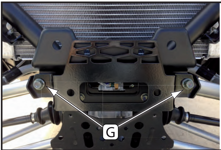
“Figure 10” Fairlead Bracket Install
