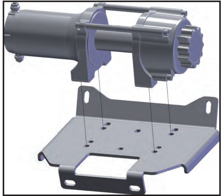
“Figure 8” Winch Install
