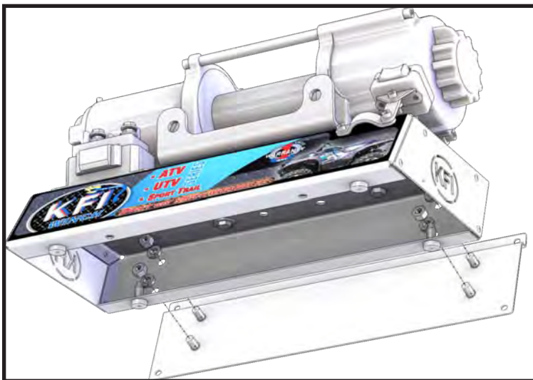
"Figure 3" Slat Wall Plate Install
