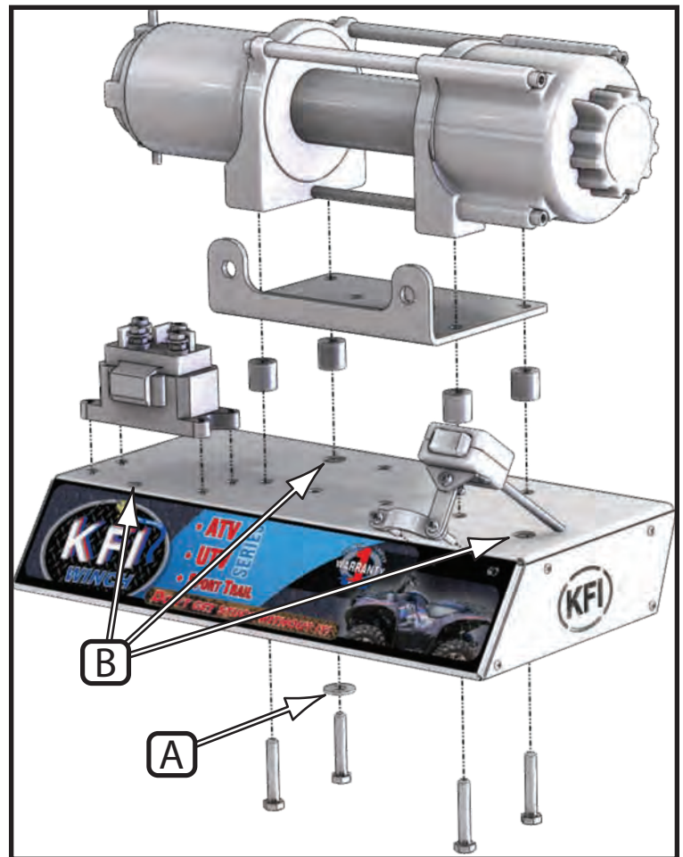
"Figure 2" Winch Install
