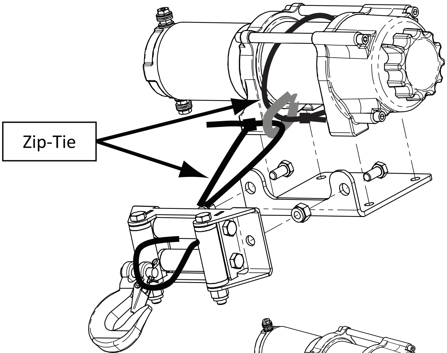
“Figure 4” Zip Tie Install
