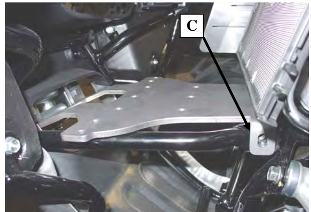
"Figure 2" Remove Middle Bumper Bolts and attach mount
